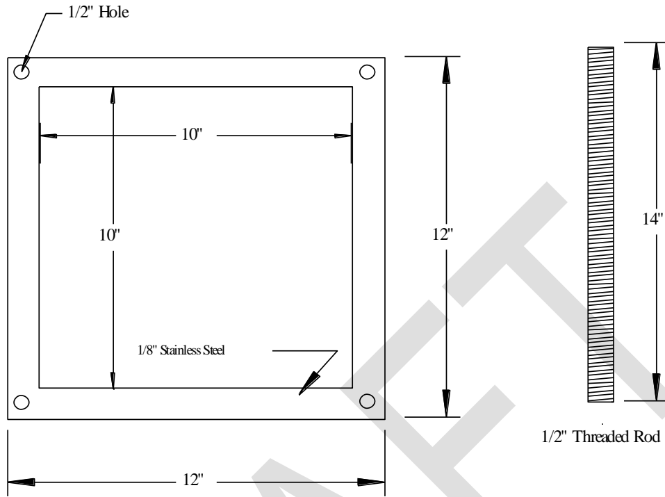
Rectangular Metal Retaining Ring
